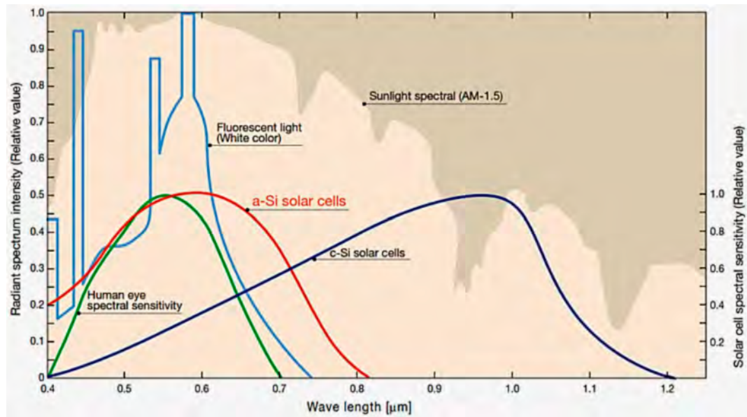
Figure 5. Comparison of relative radiant spectra of sunlight vs. artificial light from incandescent bulbs and fluorescent lamps.
