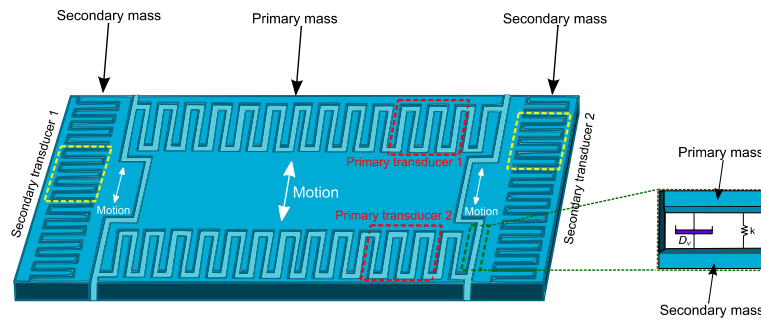
Figure 10. Electrostatic kinetic harvester.
