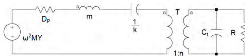
Figure 11. Equivalent circuit of an electrostatic force harvester.
