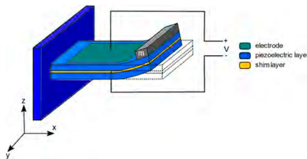
Figure 6. Piezoelectric kinetic harvester.
