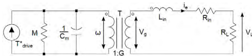
Figure 21. Micro-wind/water harvester equivalent circuit schematic.
