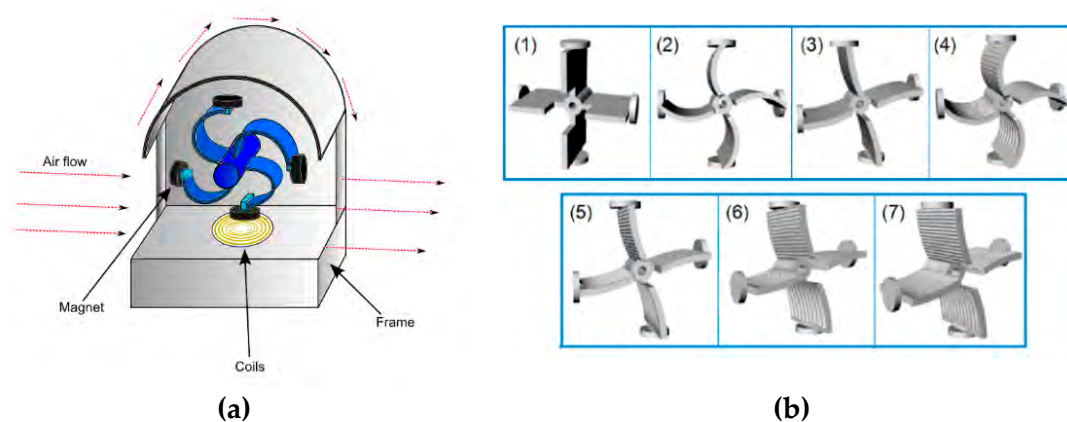
Figure 22. Micro wind harvester. (a) Micro wind harvester; (b) Wind harvester possible blades topologies.
