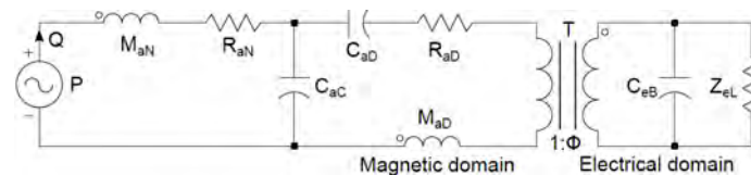
Figure 25. Equivalent circuit of an acoustic harvester.
