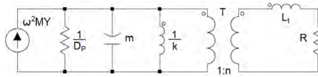
Figure 9. Equivalent circuit of an electromagnetic force harvester.
