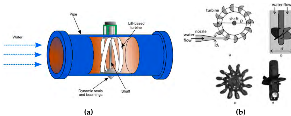
Figure 23. Examples of water flow harvester. (a) Water flows energy harvester; (b) Usual generators design.
