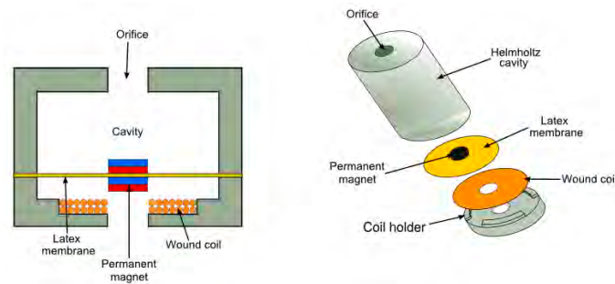
Figure 24. Acoustic noise harvester.
