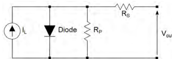
Figure 4. Photovoltaic harvester equivalent circuit.
