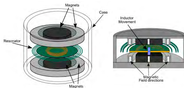
Figure 8. Magnetic kinetic harvester.
