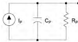
Figure 14. Pyroelectric harvester equivalent circuit.
