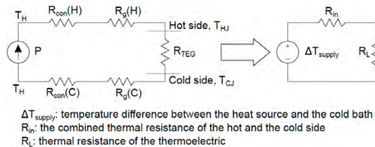
Figure 16. Equivalent electro-thermal circuit of a thermoelectric energy harvesting device.
