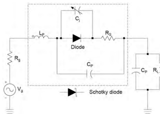
Figure 20. The equivalent circuit of a RF harvester and an integrated rectifier.
