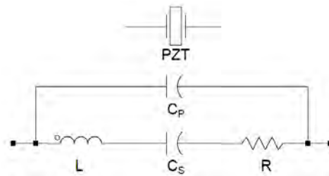
Figure 7. Quartz piezoelectric harvester equivalent circuit.
