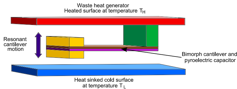
Figure 13. Pyroelectric harvester.
