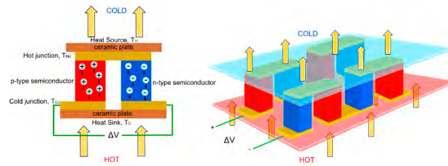
Figure 15. Thermoelectric harvester.
