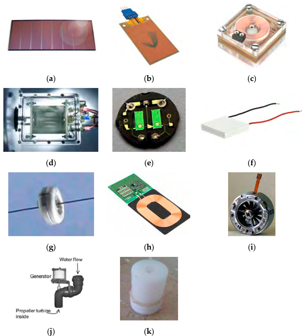
Figure 1. Energy harvesters' technologies. (a) Photovoltaic; (b) Piezoelectric; (c) Electromagnetic; (d) Electrostatic; (e) Pyroelectric; (f) Thermoelectric; (g) Magnetic; (h) RF; (i) Wind flow; (j) Liquid flow; (k) Acoustic noise.
