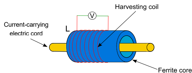
Figure 17. Magnetic harvester.
