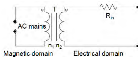
Figure 18. Equivalent circuit of a magnetic harvester with ideal impedance matching.
